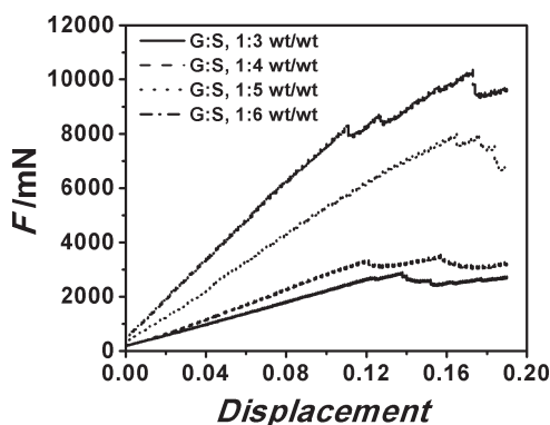
Figure 3. Force-displacement curves for microcapsules prepared at varying gelatin-shellac proportions. The reported values represent mean of five measurements, the standard deviation was less than 5% in all cases. (gelatin:shellac = G:S).
