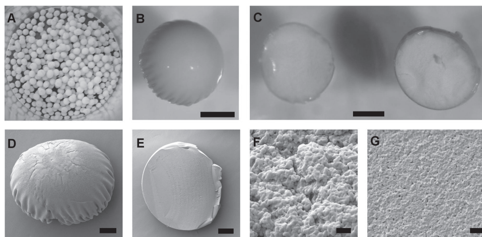
Figure 2. A) Photograph of microcapsules after minutes of formation. B,C) Optical microcopy images of an intact and cross-sectioned microcapsules (scale bars = 500 \mu\text{m} ). D,E) SEM images of intact and cross sectioned microcapsule (scale bars = 100 \mu\text{m} ). F,G) Magnification of the surface and internal structure respectively (scale bars = 200 nm).
