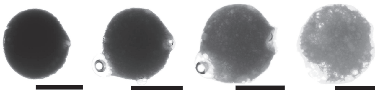
Figure 8. Microscopic images showing temperature triggered release of encapsulated aromatic oil with respect to the temperature (scale bars = 400 \mu\text{m} ). Microcapsules were prepared at GL:SL, 1:6 wt/wt with 10 wt% d-Limonene. Temperature from left to right: 20, 60, 70 and 80 °C.
