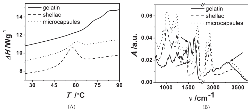
Figure 4. A) DSC heat flow graphs and B) FT-IR spectra for gelatin, shellac and microcapsules prepared using GL:SL ratio of 1:6 wt/wt.
