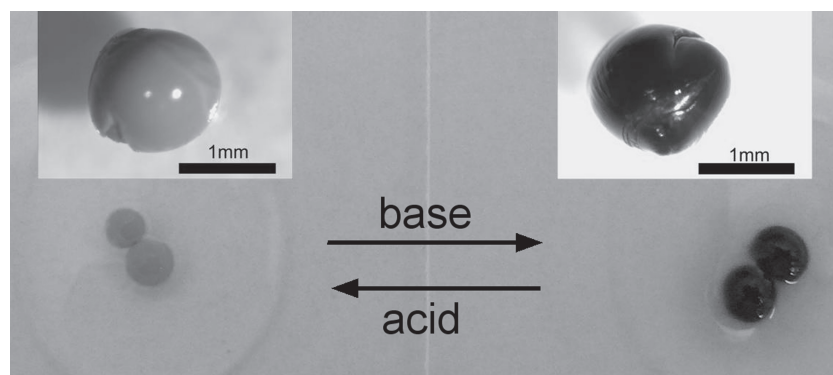
Figure 7. The photograph showing the acid-base color changes of alizarin loaded microcapsules between yellow and blue. Insets: Colored images of microcapsule from Leica Macroscope. Color images are provided as Figure S2 (Supporting Information).
